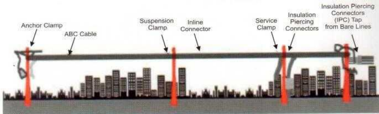
Typical LT Aerial Bunched Cable Network
